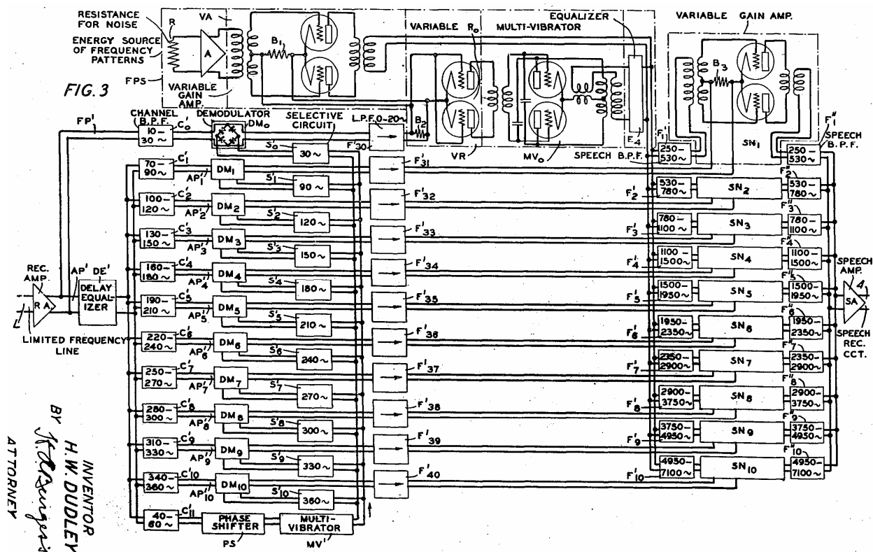
Figure 9. Dudley patent, signal transmission.
